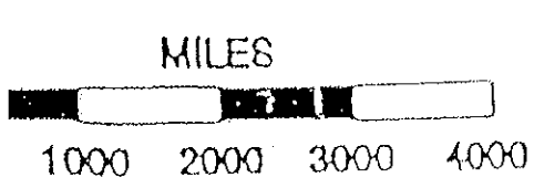
World Physical Map
