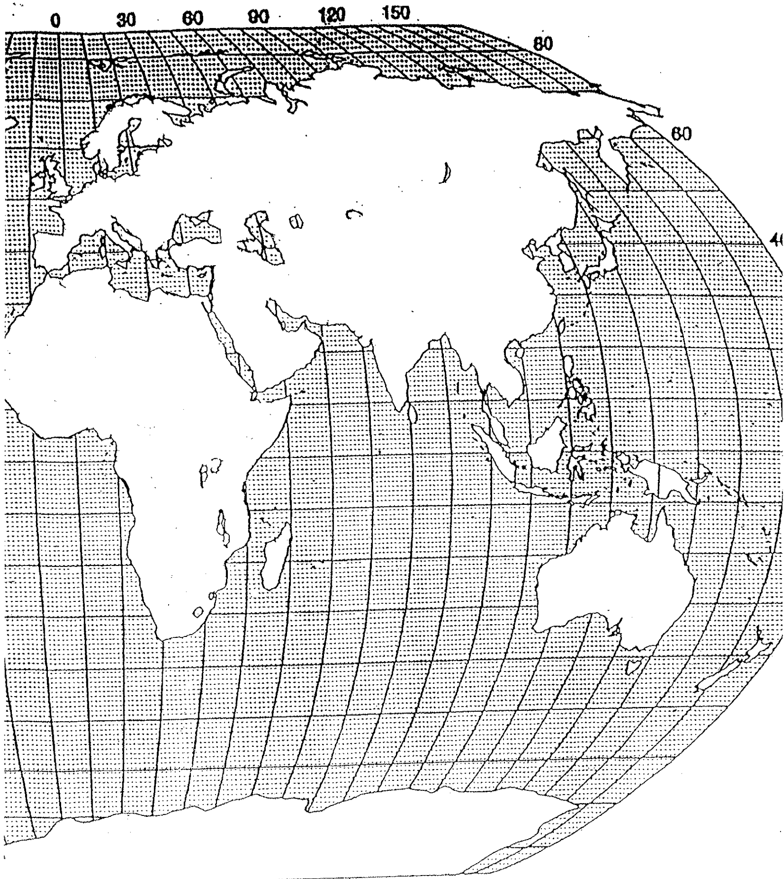
World Physical Map
